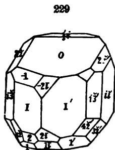
Anorthite.
